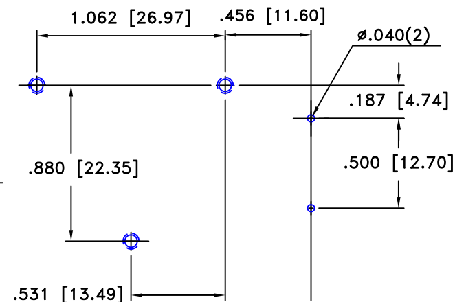
PCB LAYOUT
