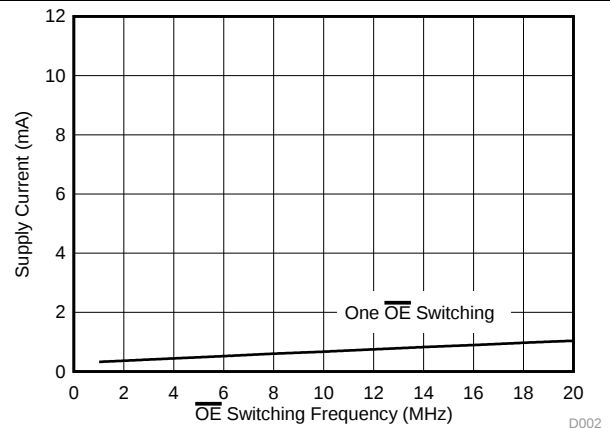
Figure 2. Typical Supply Current vs OE Switching Frequency
