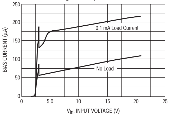
Figure 3. Input Current
