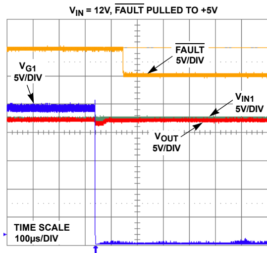
FIGURE 27. MOSFET GATE TO SOURCE FAULT
