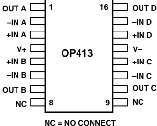
16-Lead Narrow-Body SOL (S Suffix)
