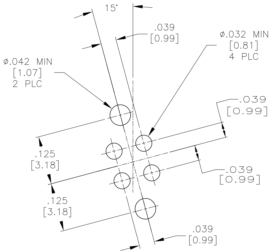
DETAIL T SCALE NTS 4 PLC
