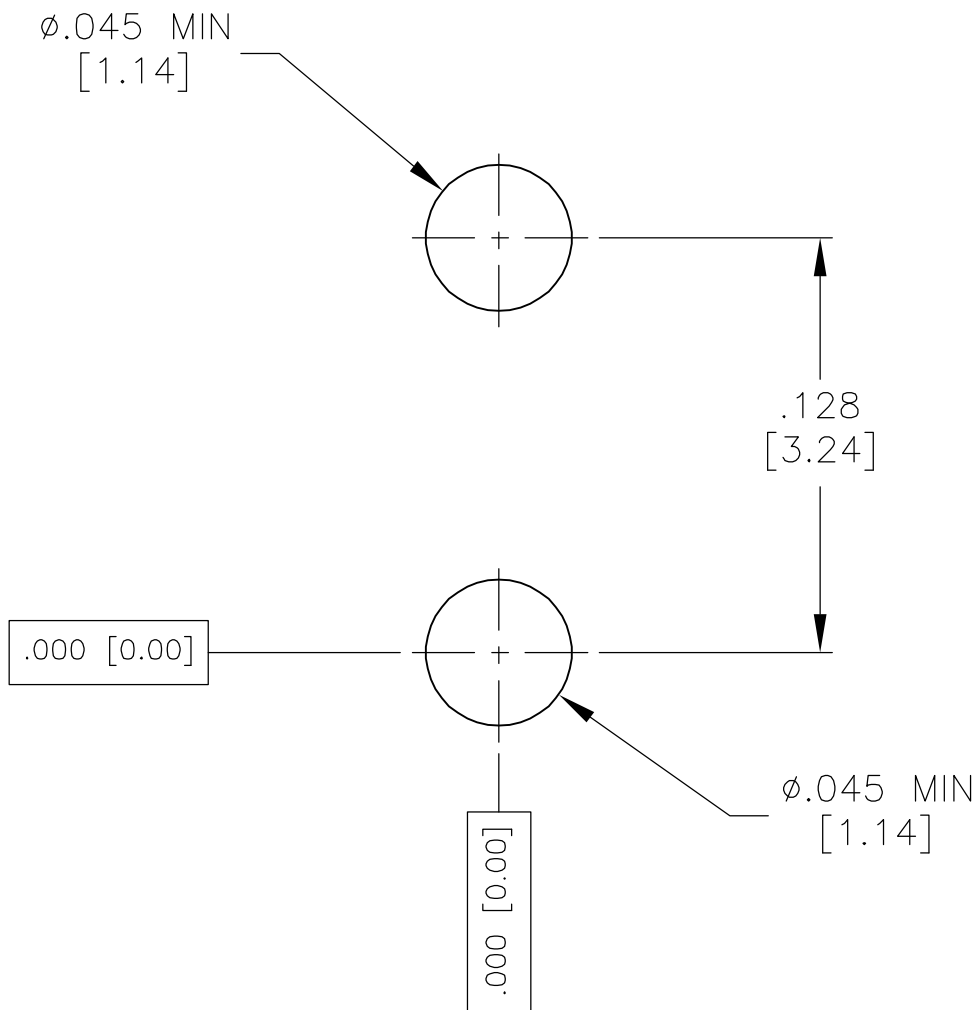
DETAIL S SCALE NTS 10 PLC
