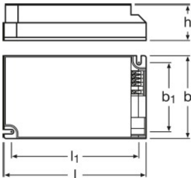
Product line drawing OTp DALI 35/220...240/700 HD
