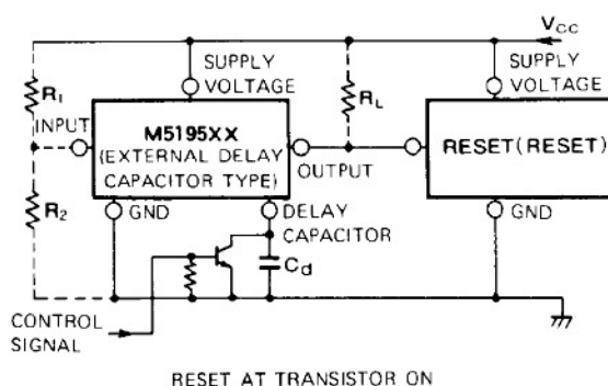
(b) Reset at transistor ON
