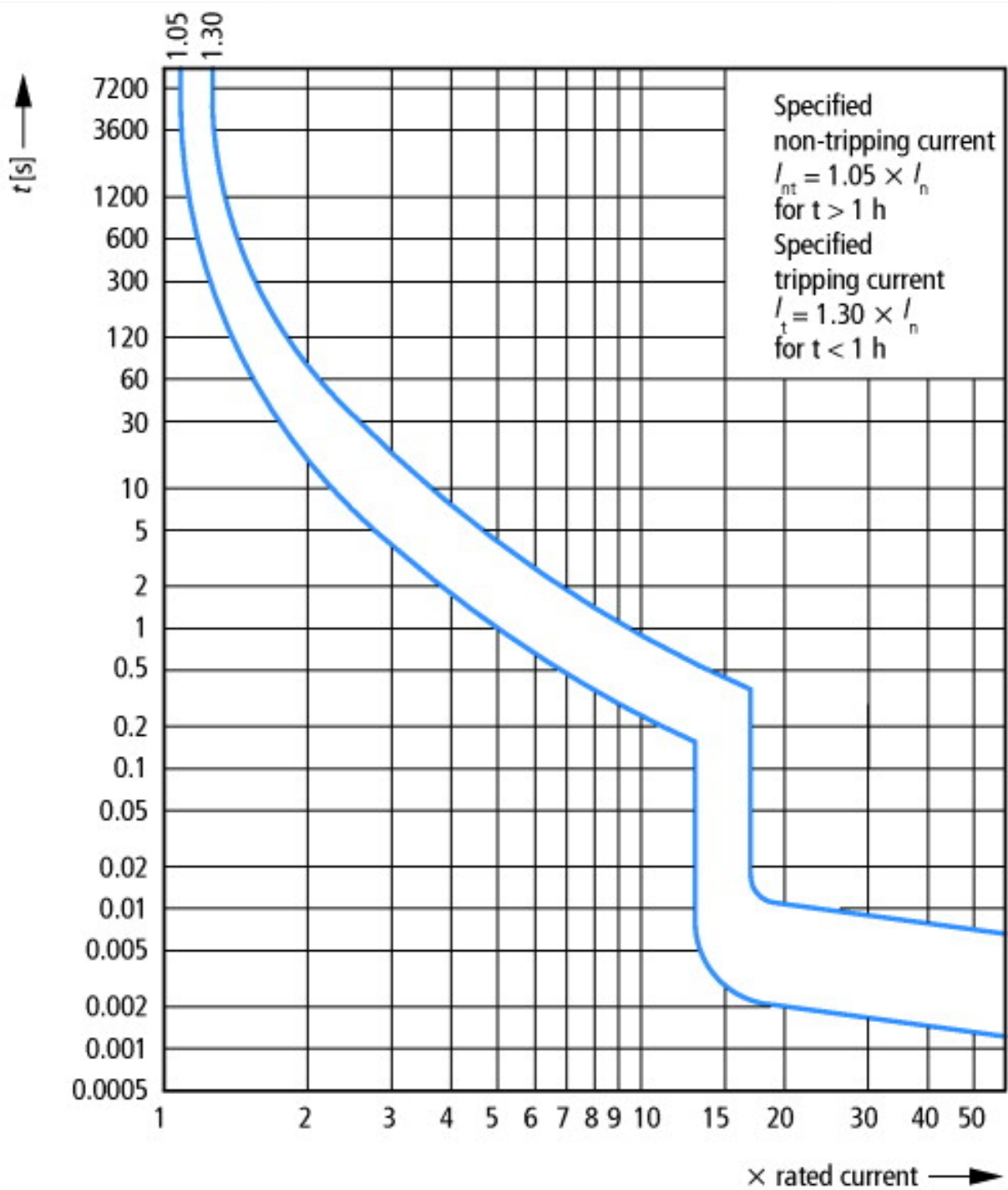
Tripping characteristic FAZ at 30 °C: S according to IEC/EN 60947
