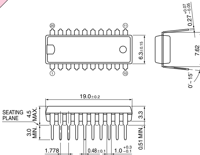
TYPE 20P4B 20pin 300mil DIP
