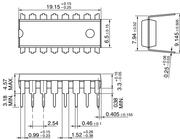
TYPE 16P4X 16pin 300mil DIP
