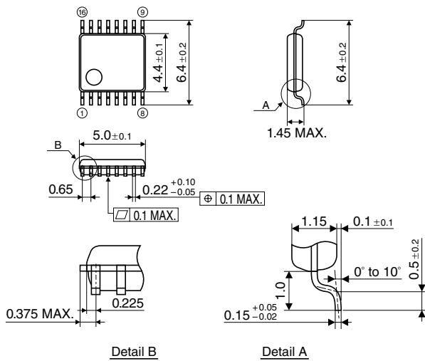
TYPE 16P2E-A 16pin 225mil SSOP
