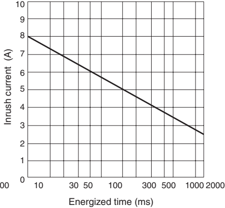
G3R-OD201SN-UTU
