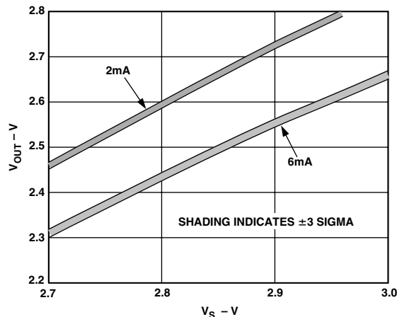
TPC 22. Distribution of Maximum OUT Voltage vs. Supply Voltage with 2 mA and 6 mA Loads, 3 Sigma to Either Side of Mean, AD8316 Sourcing
