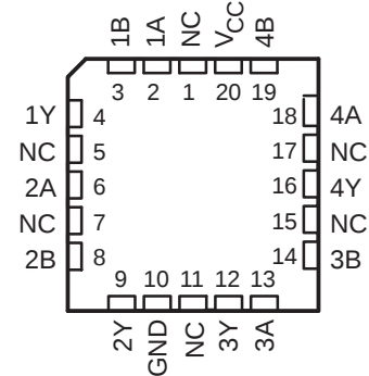
SN54ALS32, SN54AS32 . . . FK PACKAGE (TOP VIEW)
