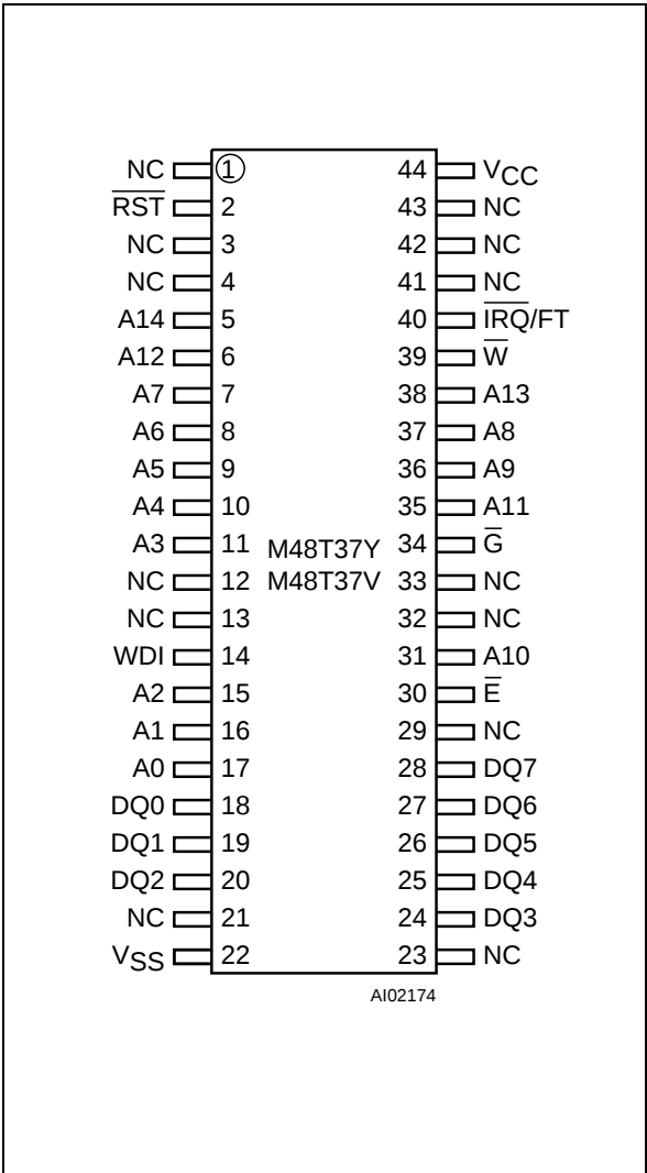
Figure 3. SOIC Connections
