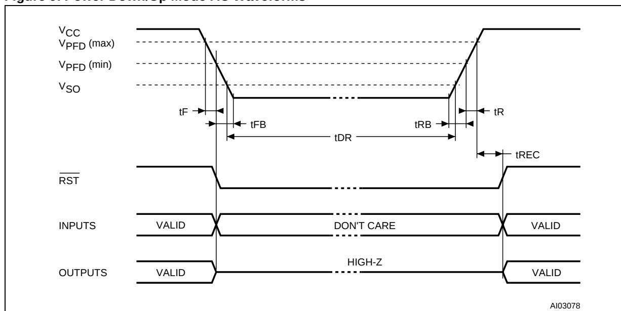
Figure 9. Power Down/Up Mode AC Waveforms
