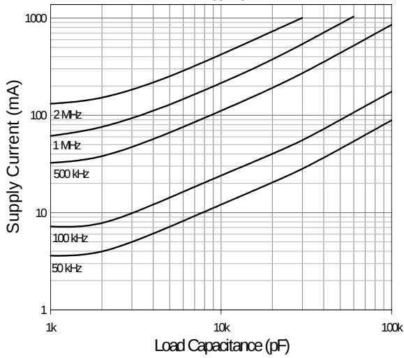
Fig. 13 Supply Current vs. Load Capacitance V_{CC}=12V
