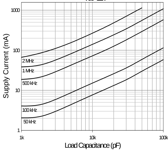
Fig. 15 Supply Current vs. Load Capacitance V_{CC}=8V
