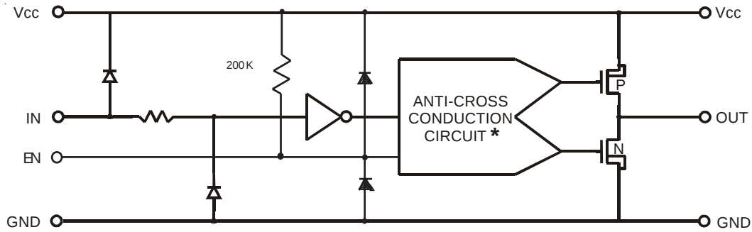
Figure 1 - IXDD514 14A Non-Inverting Gate Driver Functional Block Diagram
