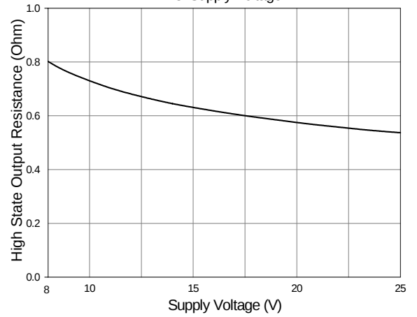
High State Output Resistance vs. Supply Voltage
