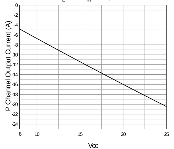
V_{CC} vs. P Channel Output Current C_L = 1\mu F V_{IN} = 0.5V @ 1kHz
