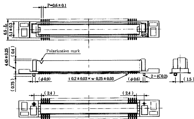
[FX8C- **/ **P11-SVJ]
