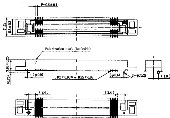
[FX8C- **/ **S11-SVJ]
