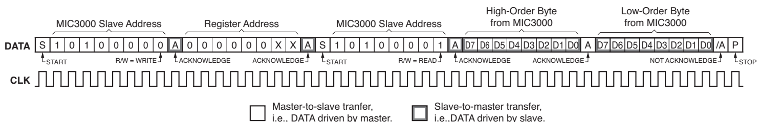
Figure 23. Read_Word Protocol
