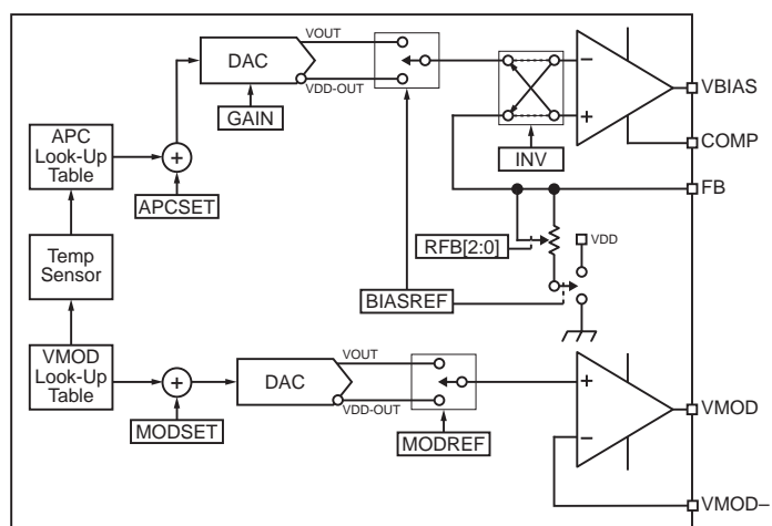
Figure 3. MIC3000 APC and Modulation Control Block Diagram
