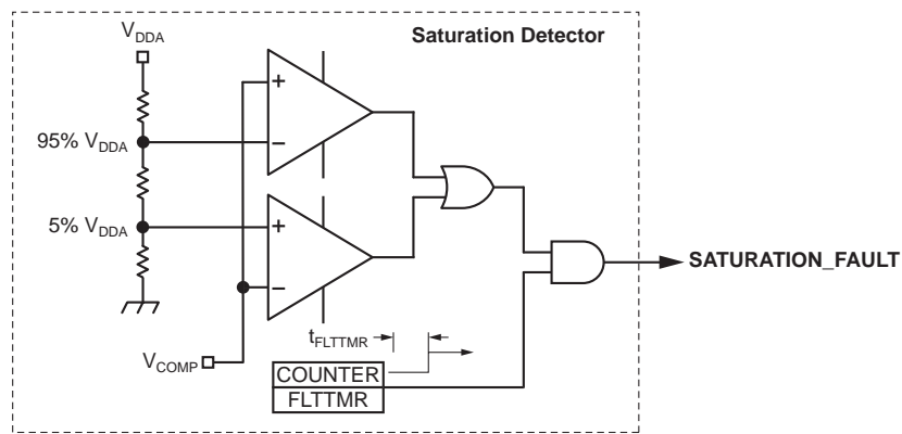
Figure 9. Saturation Detector
