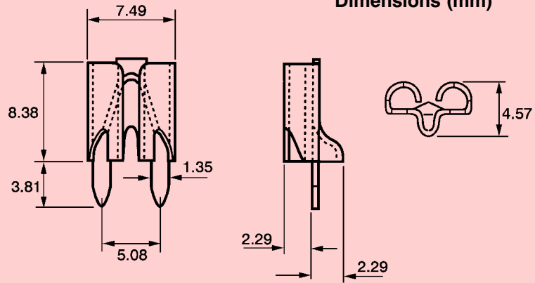
Dimensions (mm)
