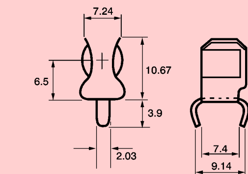
Dimensions (mm)
