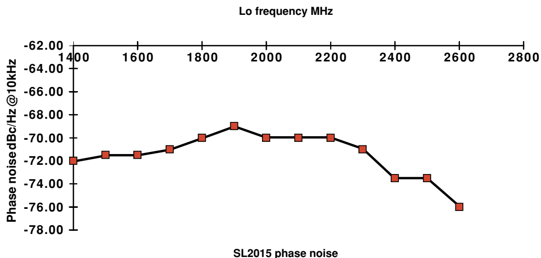
Figure 5 - LO phase noise variation with frequency (typical)
