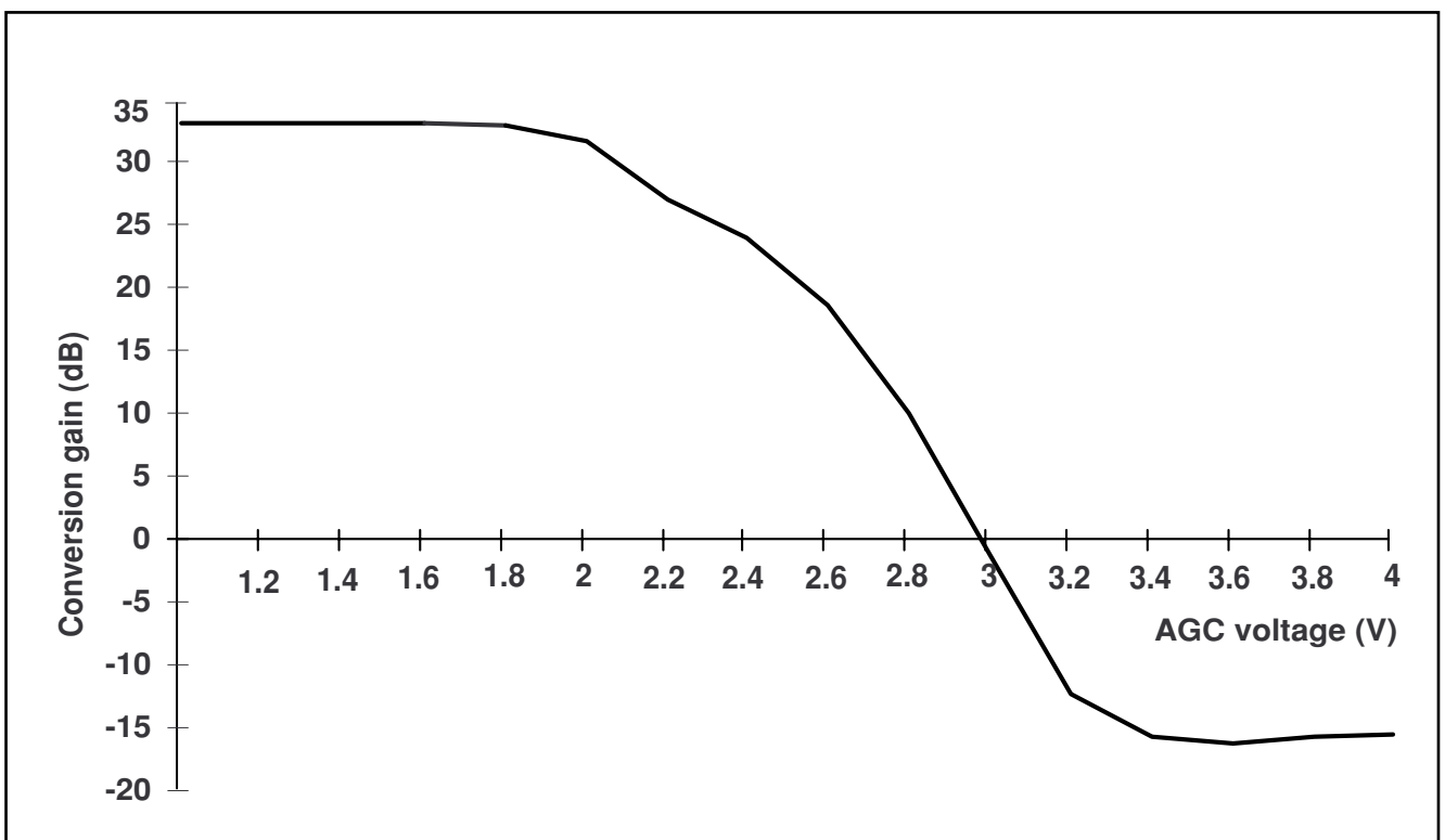
Figure 9 - Gain variation with AGC voltage (typical)
