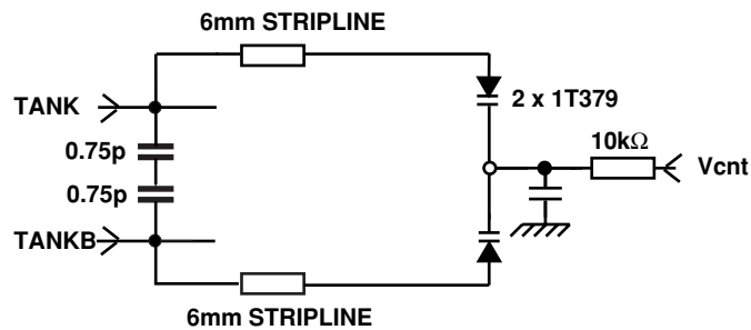
Figure 4 - VCO application circuit
