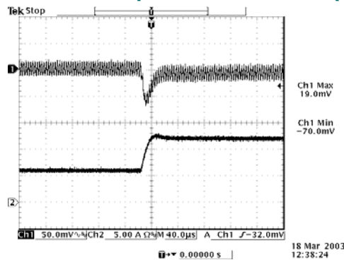
50% to 100% load 3.3 Vdc Input 1.8 Vdc Output
