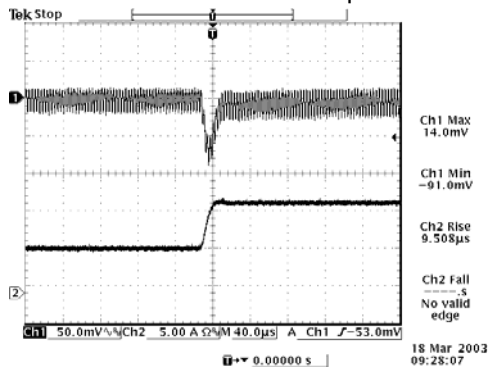
50% to 100% load 5 Vdc Input 1.8 Vdc Output
