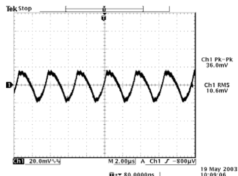
5 Vdc Input 1.8 Vdc Output
