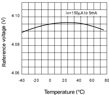
Temperature Drift
