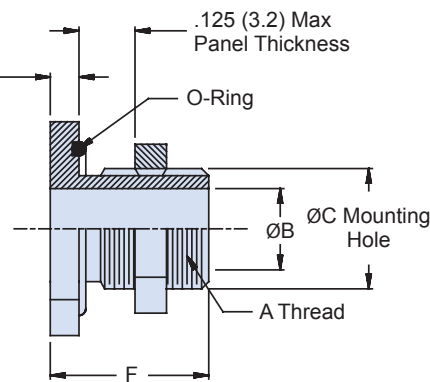
Bulkhead Adapters 710-100/101/372
