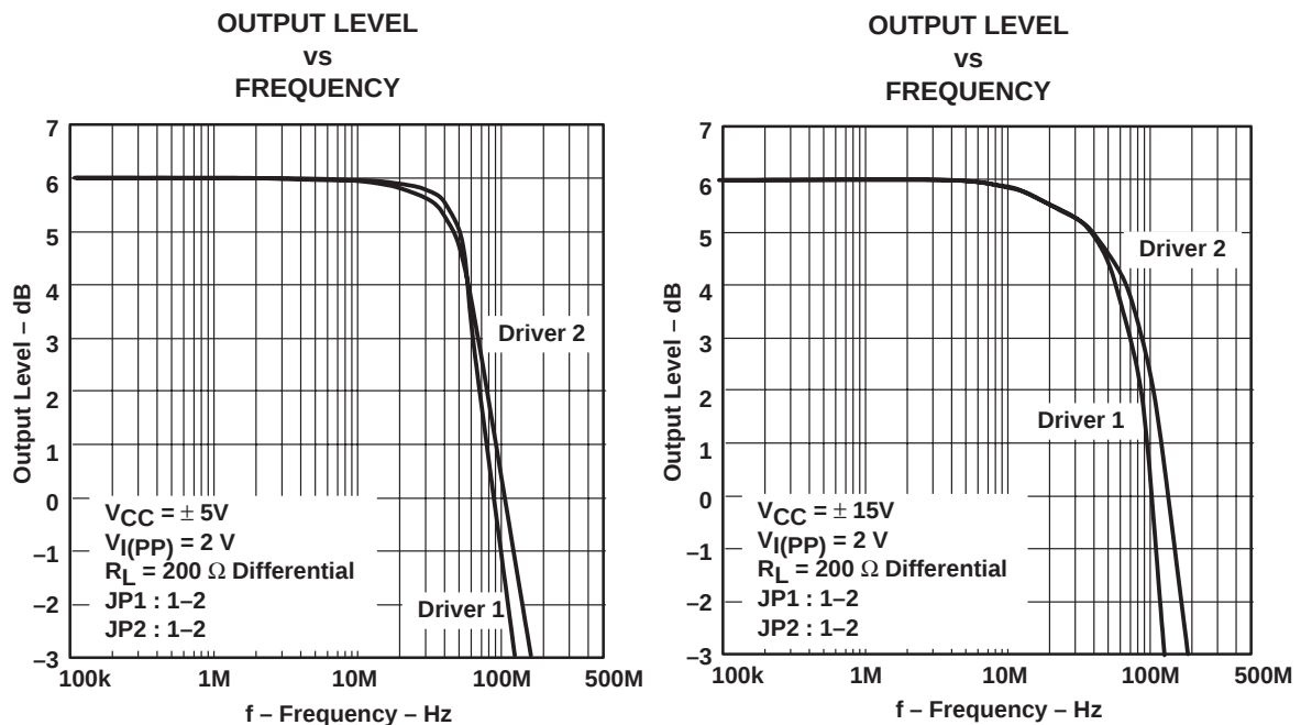
Figure 1–4. THS6022 EVM Driver Frequency Response With a 50- \Omega Load
