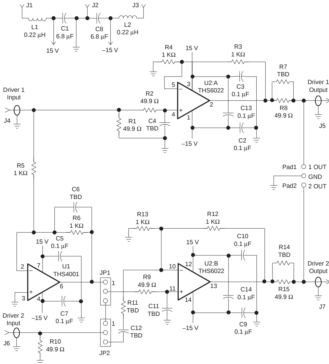
Figure 1–2. THS6022 Evaluation Module Schematic
