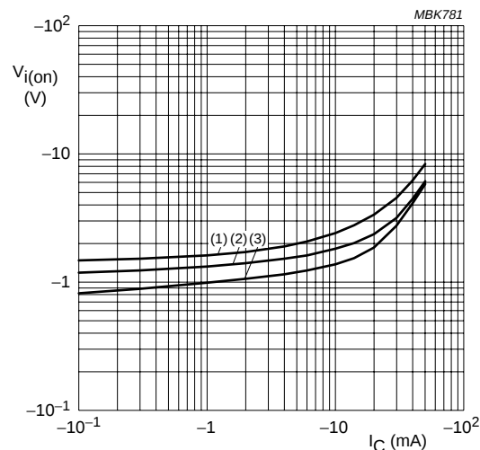
TR2 (PNP); V_{CE} = -0.3\text{ V} . (1) T_{amb} = -40^\circ\text{C} . (2) T_{amb} = 25^\circ\text{C} . (3) T_{amb} = 100^\circ\text{C} .
