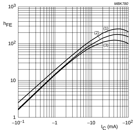
TR2 (PNP); V_{CE} = -5\text{ V} . (1) T_{amb} = 150^\circ\text{C} . (2) T_{amb} = 25^\circ\text{C} . (3) T_{amb} = -40^\circ\text{C} .
