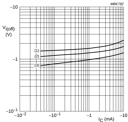
TR2 (PNP); V_{CE} = -5\text{ V} . (1) T_{amb} = -40^\circ\text{C} . (2) T_{amb} = 25^\circ\text{C} . (3) T_{amb} = 100^\circ\text{C} .
