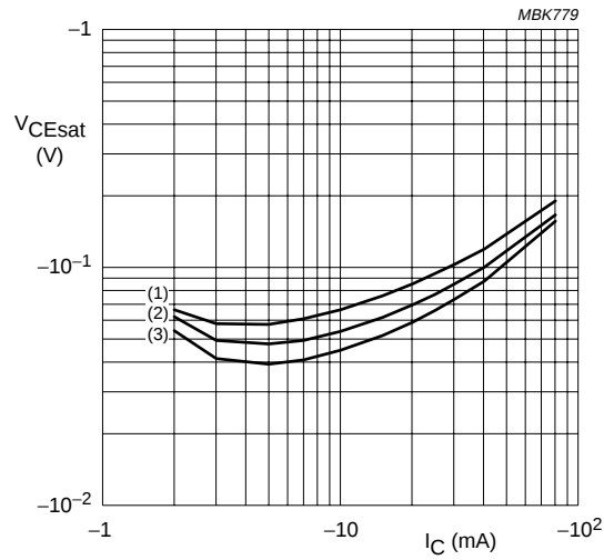
TR2 (PNP); I_C/I_B = 20 . (1) T_{amb} = 100^\circ\text{C} . (2) T_{amb} = 25^\circ\text{C} . (3) T_{amb} = -40^\circ\text{C} .
