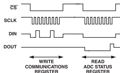
Figure 6. The Serial Interface Signals—Register Access
