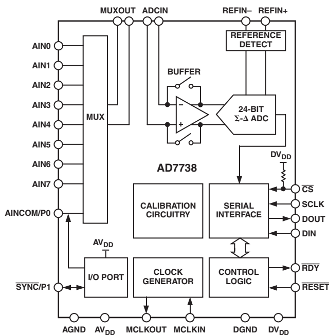
Figure 4. Block Diagram
