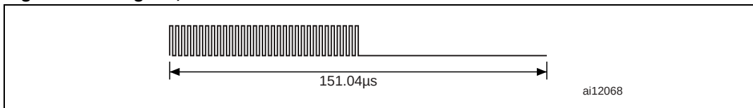
Figure 16. Logic 0, low data rate
