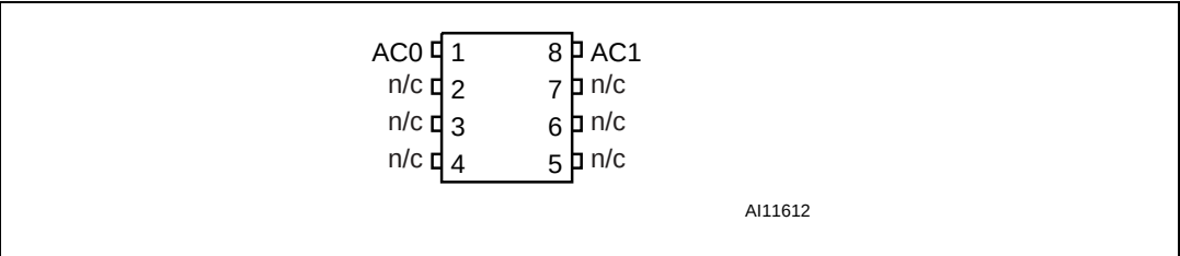
Figure 2. MLP connections
