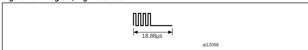
Figure 13. Logic 0, high data rate x2
