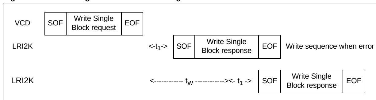
Figure 43. Write Single Block frame exchange between VCD and LRI2K
