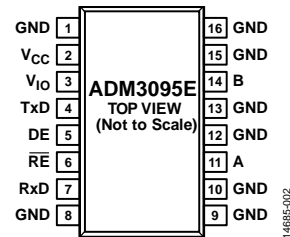
Figure 6. Pin Configuration
