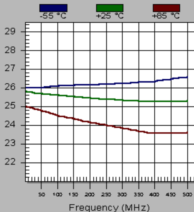
TM6523 Gain (dB)
