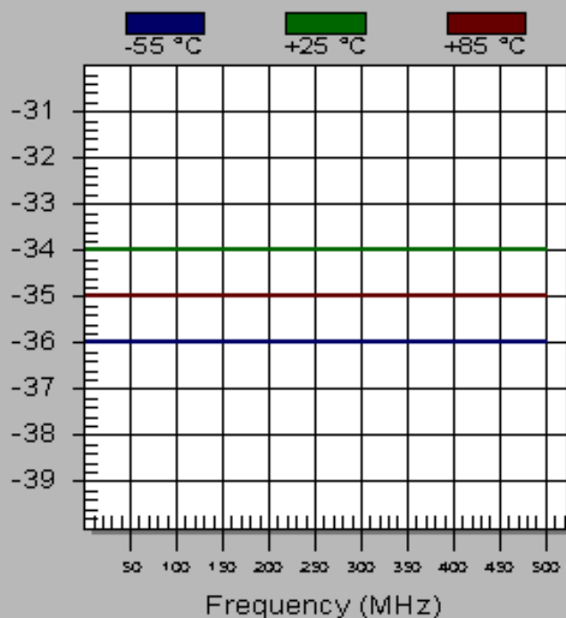
TM6523 Reverse Isolation (dB)
