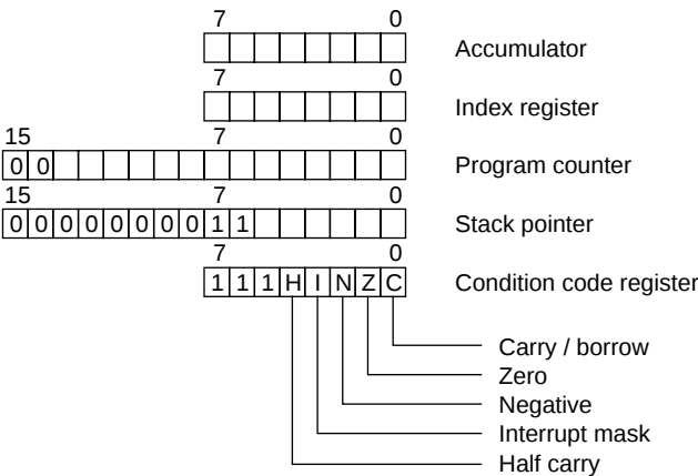
Figure 11-1 Programming model
