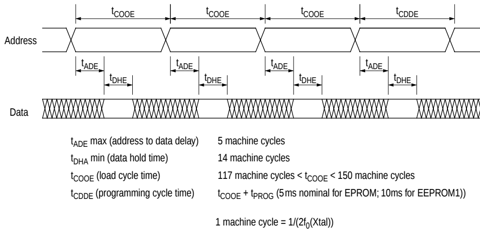
Figure B-5 Parallel EPROM loader timing diagram
