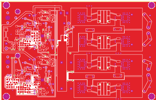
Fig.2. Top Copper
