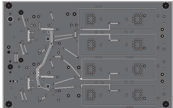
Fig.3. Bottom Copper
