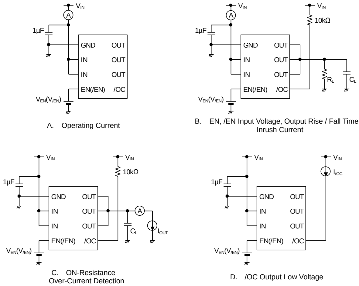
Figure 1. Measurement Circuit
