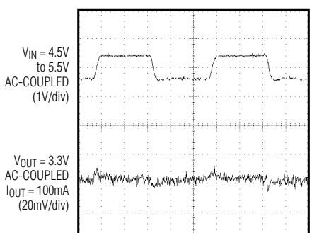
LINE-TRANSIENT RESPONSE
