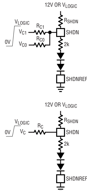
Figure 4. Providing Logic Input Control of Operating Current
