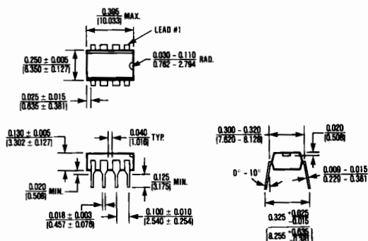
8 Lead Plastic DIP (PA)
