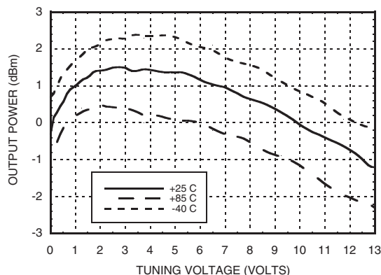
RFOUT/2 Output Power Power vs. Tuning Voltage, Vcc= +5V
