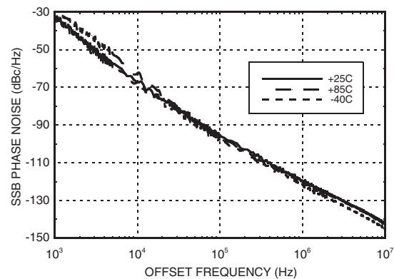
SSB Phase Noise @ V_{\text{tune}} = 5\text{V}
