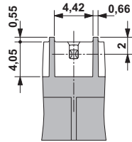
Dimensioned drawing
