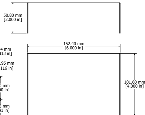
BOTTOM/TOP ENCLOSURE
