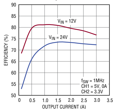
3.3V Efficiency
