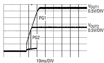
Absolute Start-Up
