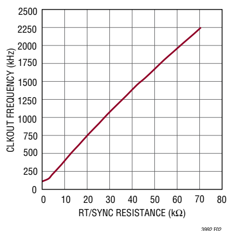
Figure 2. Switching Frequency vs RT/SYNC Resistance
