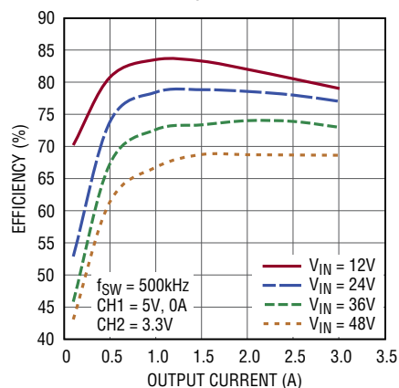
3.3V Efficiency
