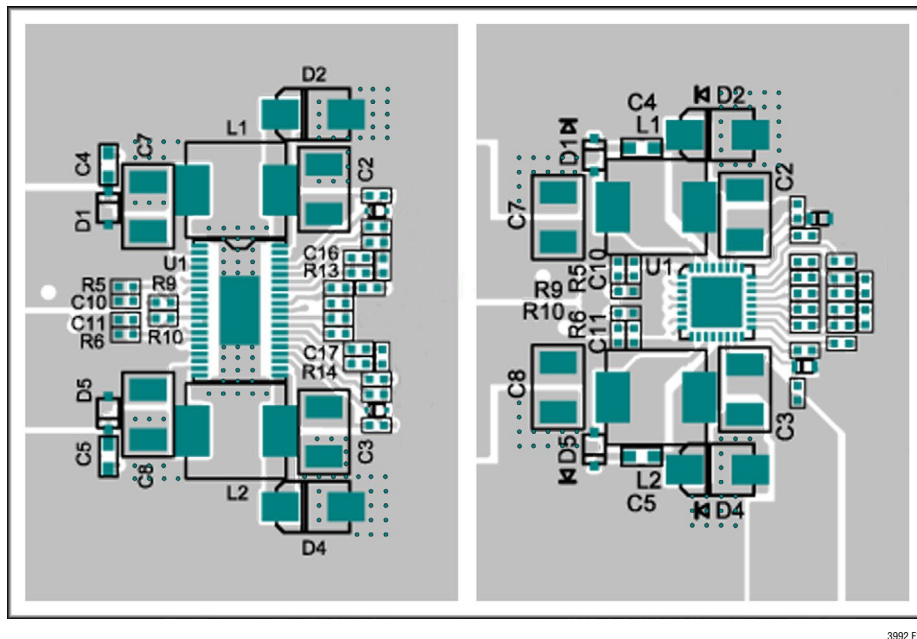
Figure 19. PCB Top Layer and Component Placement for TSSOP and QFN Packages
