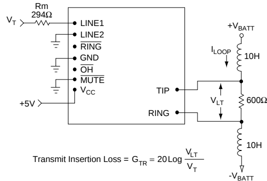
1. CYG21XX Transmit Insertion Loss
