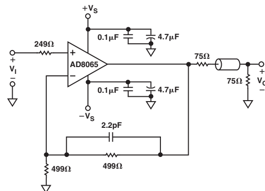
Figure 11. Video Buffer
