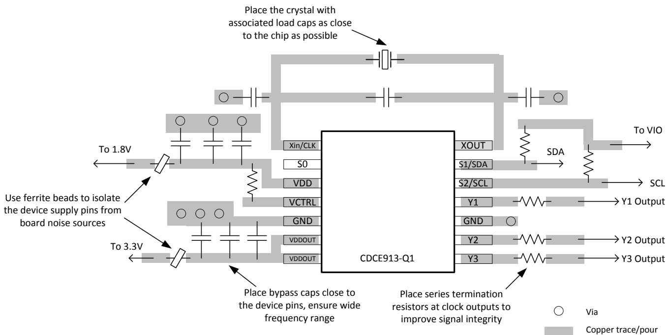
Figure 24. Annotated Layout
