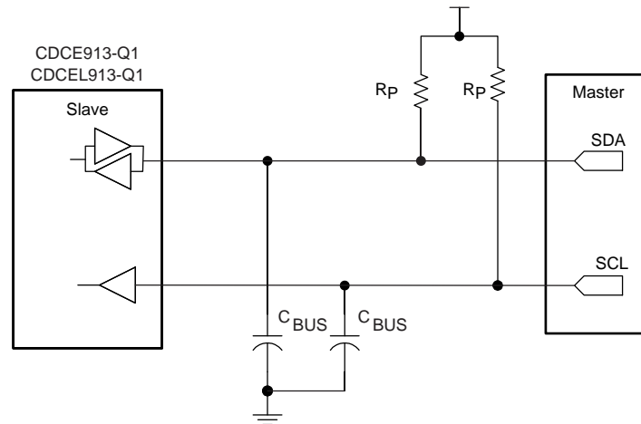
Figure 7. I²C Hardware Interface
