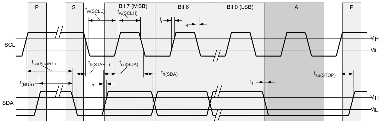
Figure 13. Timing Diagram for I²C Serial Control Interface
