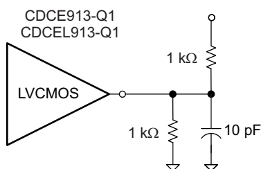
Figure 4. Test Load
