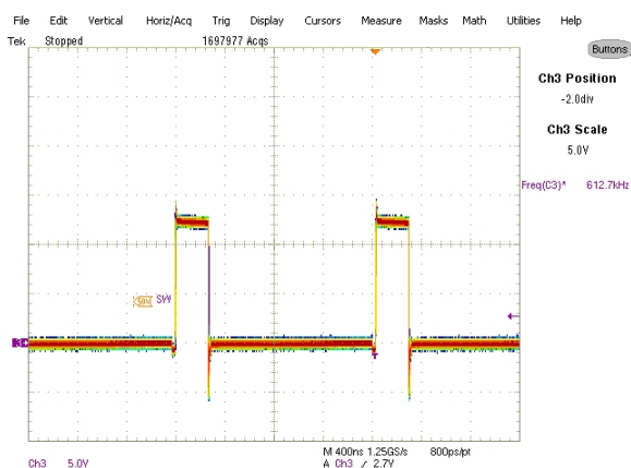
Fig. 13: Inductor node at 6A load Ch 3 :SW
