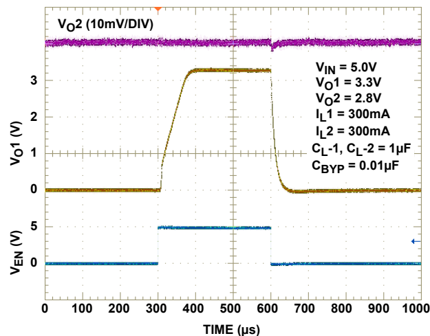
FIGURE 12. TURN-ON/TURN-OFF RESPONSE
