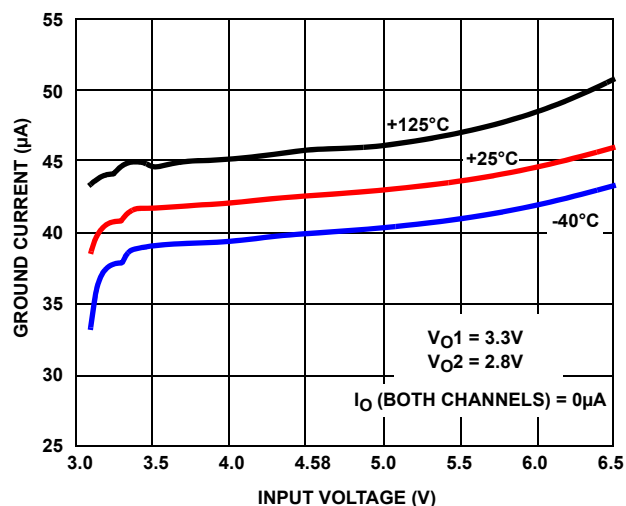
FIGURE 8. GROUND CURRENT vs INPUT VOLTAGE
