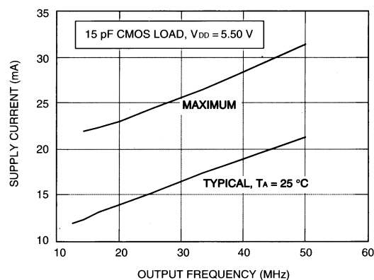
Figure 8. Supply Current vs. Output Frequency
