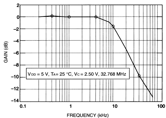
Figure 10. VCXO Input Frequency Response
