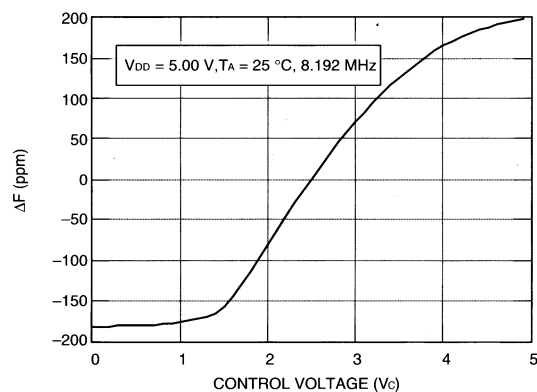
Figure 11. Output Frequency vs. Control Voltage
