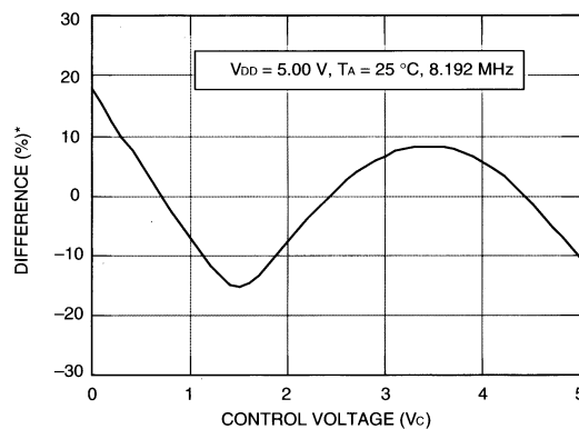
Figure 12. VCXO Linearity (Deviation From Best Linear Fit)
