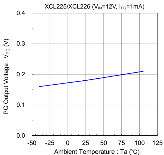
(15) PG Output Voltage vs. Ambient Temperature
