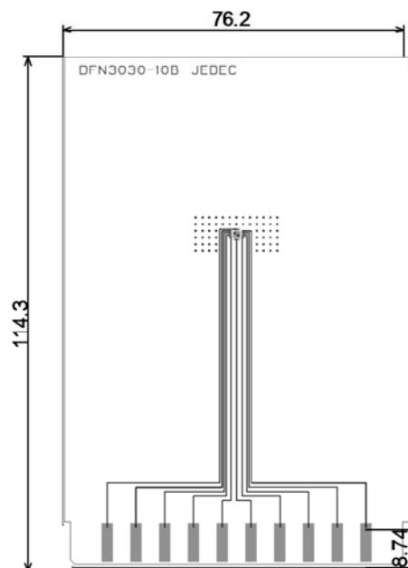
Evaluation Board (Unit: mm)
