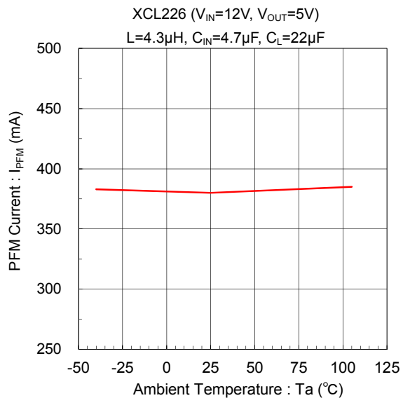
(13) PFM Current vs. Ambient Temperature
