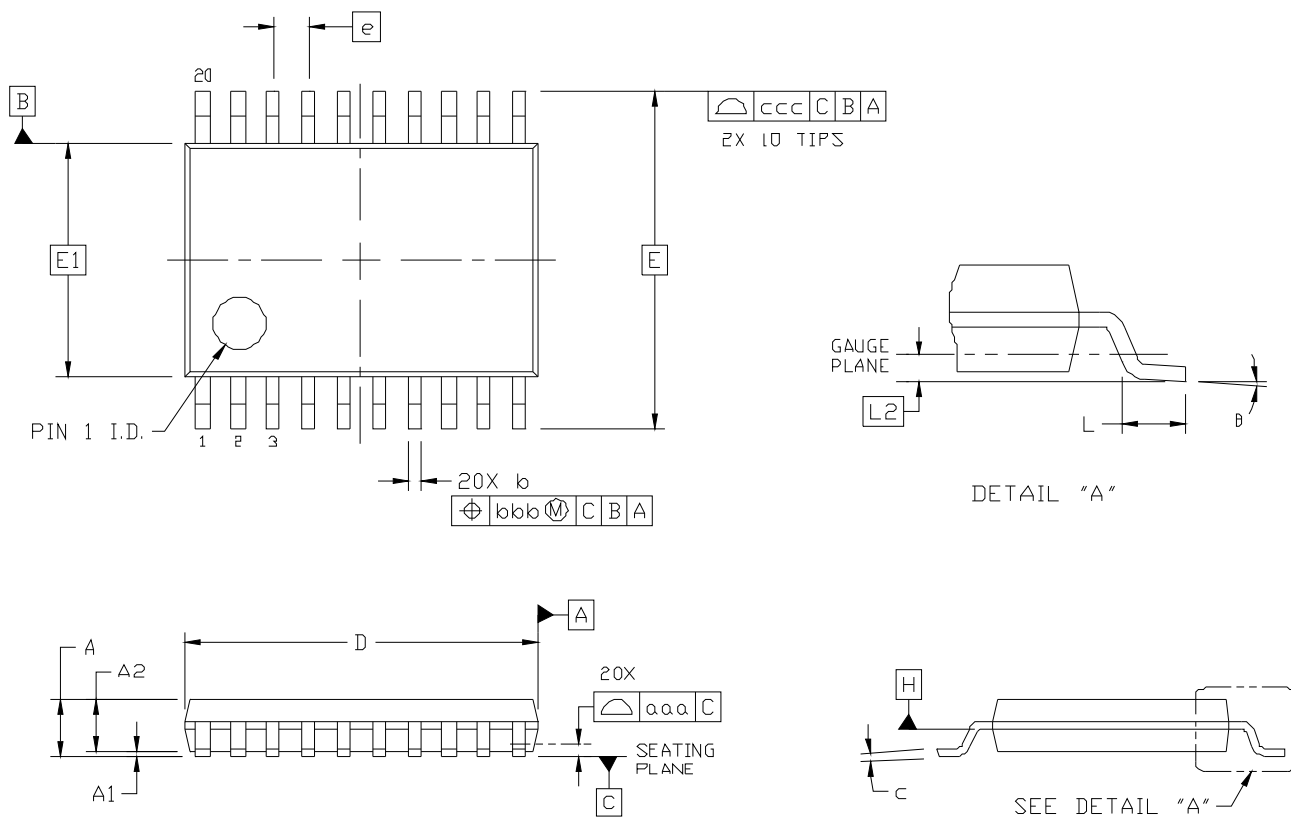
Figure 9. Si53320 20-TSSOP Package Diagram
