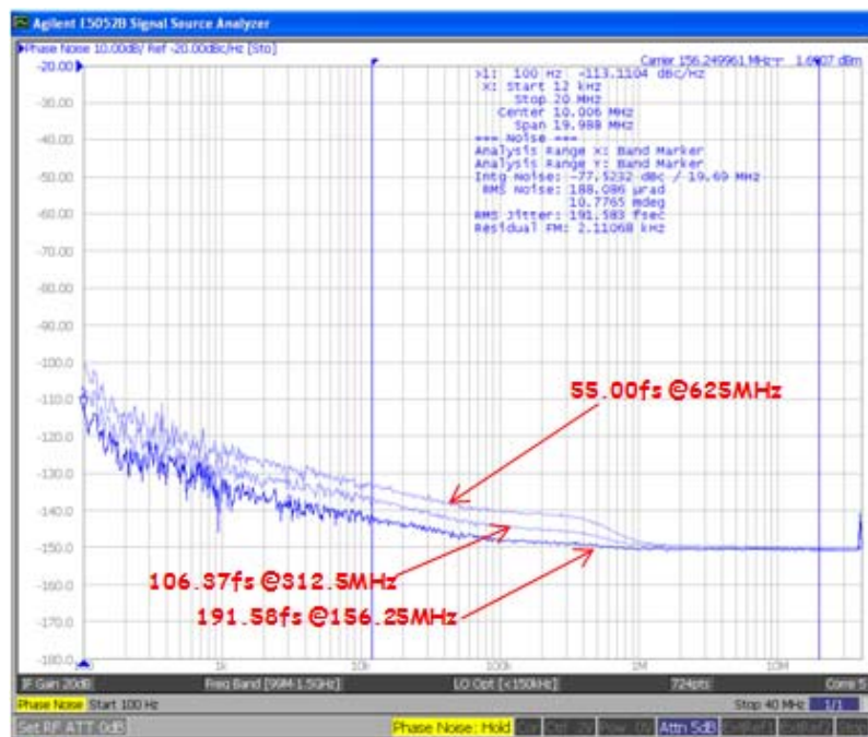
Figure 8. Si53320 Phase Noise
