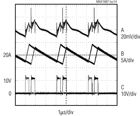
SWITCHING WAVEFORMS (OUT-OF-PHASE)
