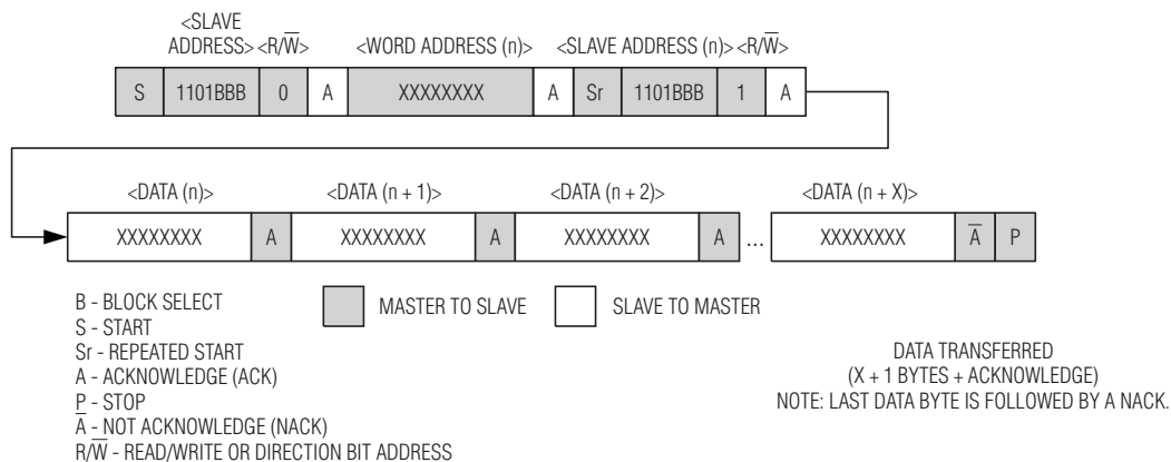
Figure 9. Data Write/Read (Write Pointer, Then Read)—Slave Receive and Transmit
