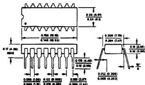
16-PIN PLASTIC DIP (SUFFIX N)
