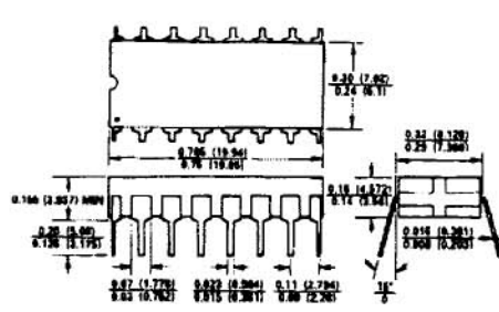
16-PIN CERDIP PACKAGE (SUFFIX Q)
