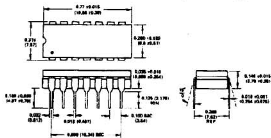
14-PIN Cerdip Package (Suffix Q)
