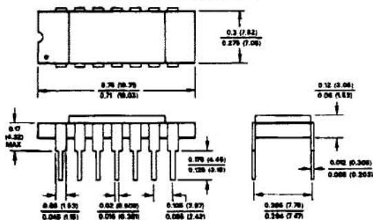
14-PIN CERAMIC DIP*
