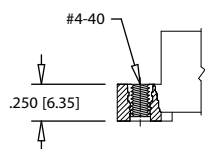
FLUSH MOUNTING WITH THREADED INSERT (T)
